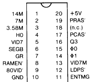
Figure 7-4 The PAL Pinouts
