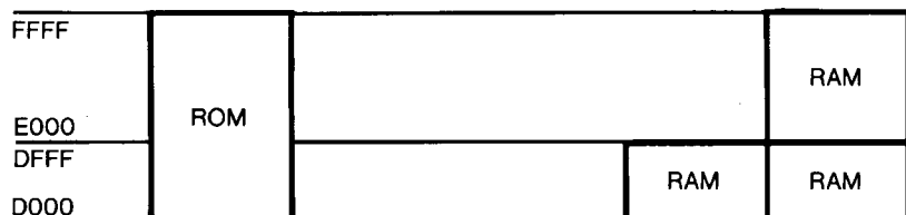
Figure 4-3 Bank-switched Memory Map
