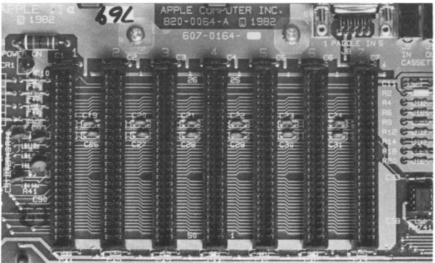
Figure 1-6 Expansion Slots
