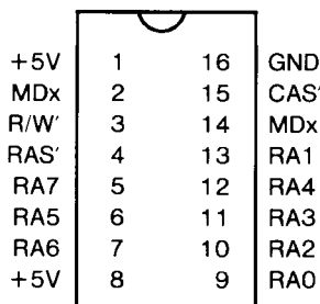
Figure 7-8 The 64K RAM Pinouts
