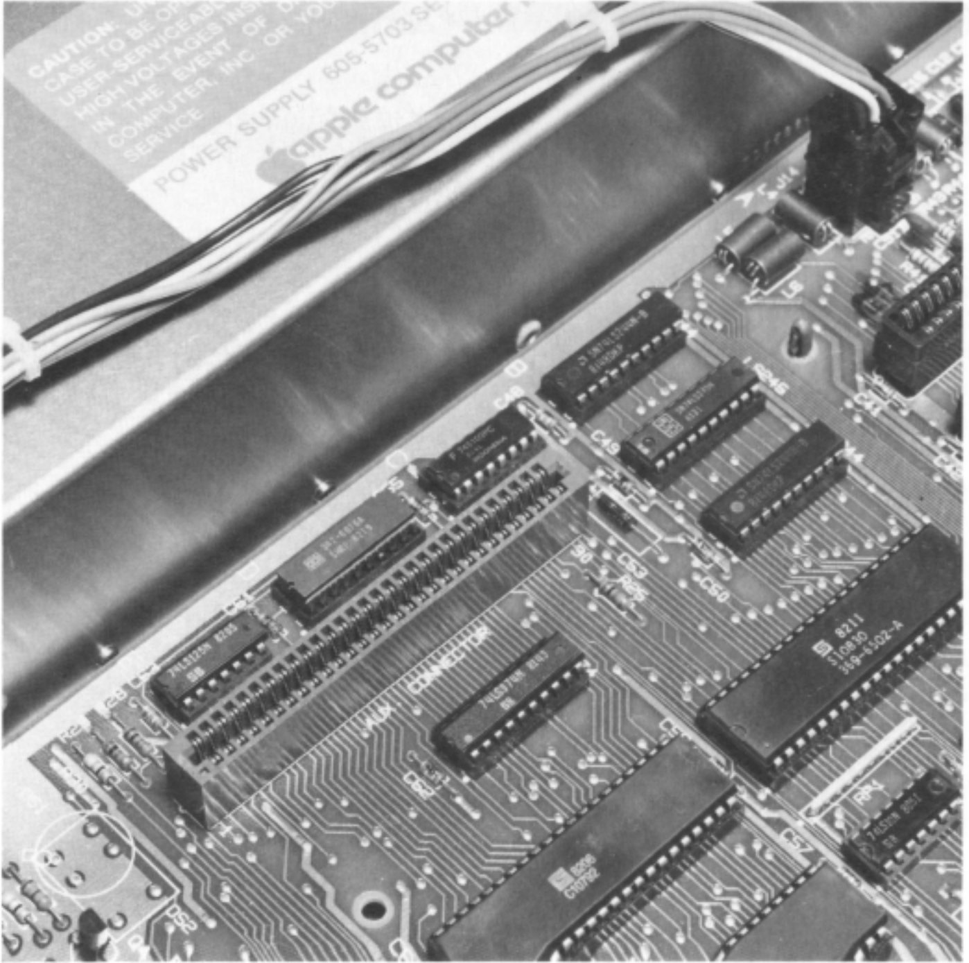
Figure 1-7 Auxiliary Slot
